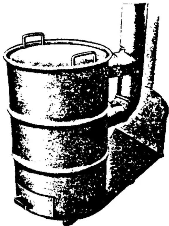
Figure 1.—The double-drum sawdust stove.
