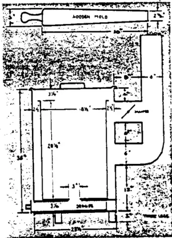
Figure 2.—Design of the experimental double-drum stove.
